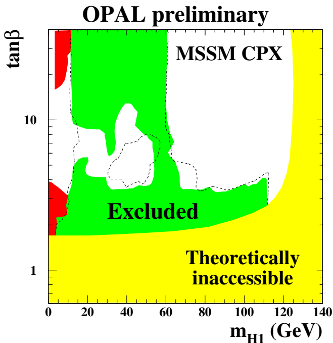
Fig. 2. Exclusion area of the CPX scenario in the \tan\beta , m_{H_1} projection from OPAL. The theoretically inaccessible area is forbidden by theory
