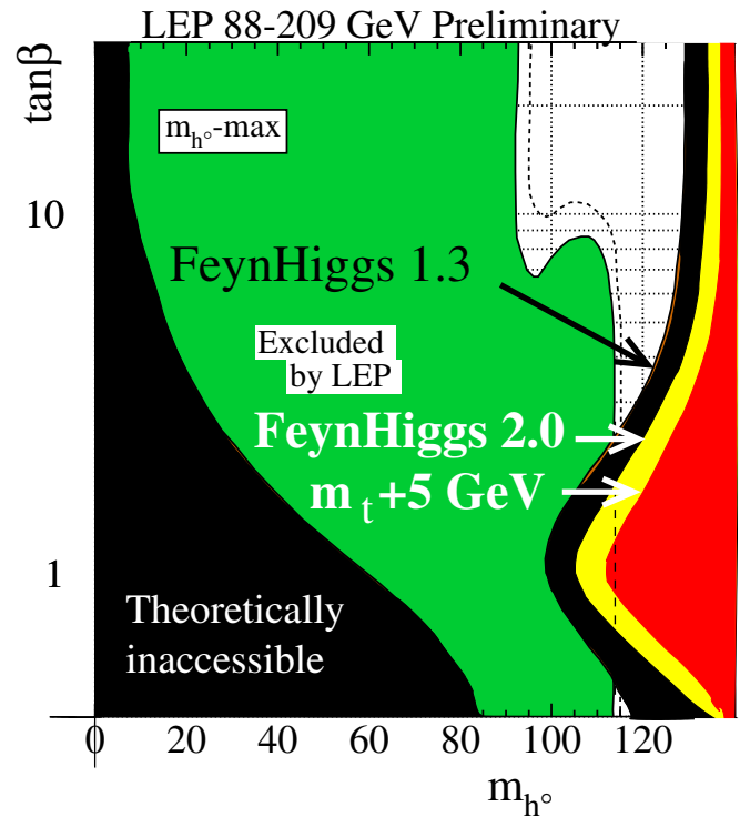
Fig. 1. Expected exclusion areas of the m_h -max scenario in the m_h , \tan\beta projection for increased upper bounds on the mass of the h boson. The experimental exclusion areas shown are those of the LEP combination 2001 [13]. The expected theoretical upper bounds for m_h given new order \alpha_t^2 loop corrections to the Higgs mass is shown in light grey (yellow) and the additional effect of a possible shift in m_t by +1\sigma is overlaid in dark grey (red). The theoretically inaccessible area is forbidden by theory
